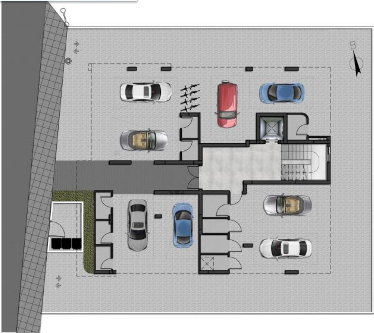
GROUND FLOOR PLAN – PARKING & STORAGE ROOMS
